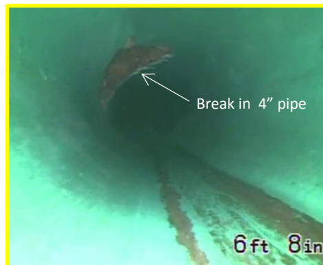
4" Drain pipe before Flow-Liner installation
